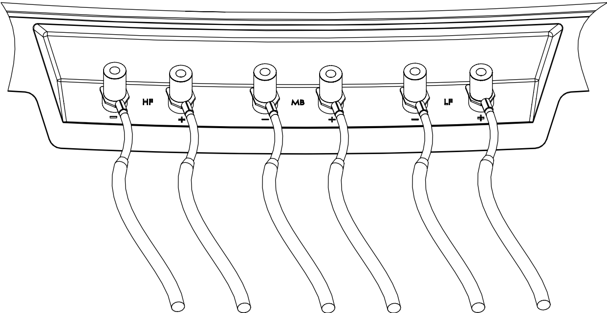
Rear Terminals
